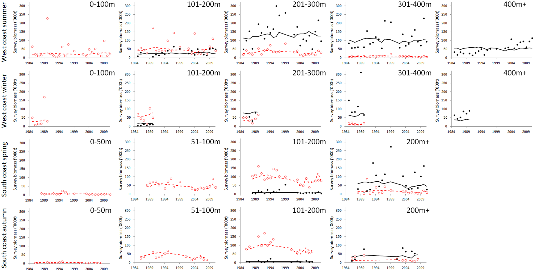
Fig. 8a: Fits to the survey biomass indices by region. M. paradoxus results are shown in black while M. capensis results are in red.
